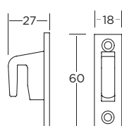
Hook plate ( HP ) can be ordered separately - code HP2a
