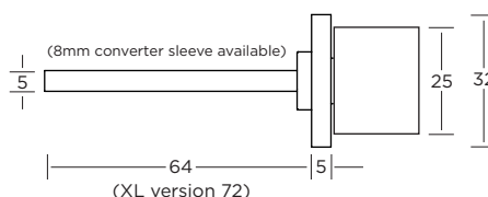
GROOVE 7833PT/AB/T47 (previously 7954)
