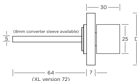
GROOVE 7833PT/T47 (previously 7478)
