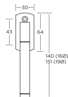
SPIRAL GRIP G05 HANDING
